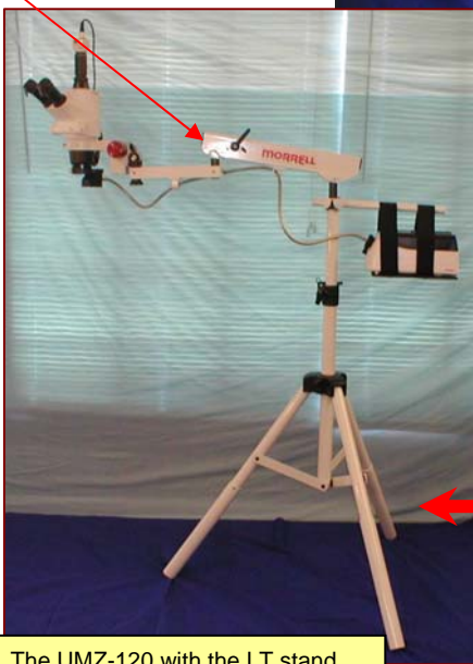
The UMZ-120 with the LT stand allows for everything to be packed in one heavy duty case. Scope, Light Source, Stand, etc...
